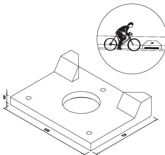
3D view of catchpit slab shown upside down
