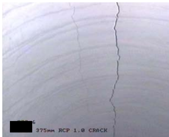
A 1mm crack at the obvert of a DN375 pipe, possibly caused by overloading of the pipe.
