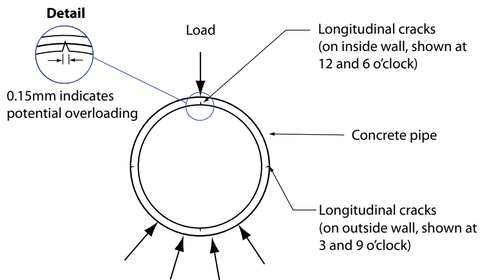
Looking at a pipe in section and the effect that overloading can have on a pipe.
