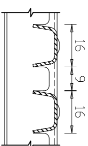
SECTION C-C
