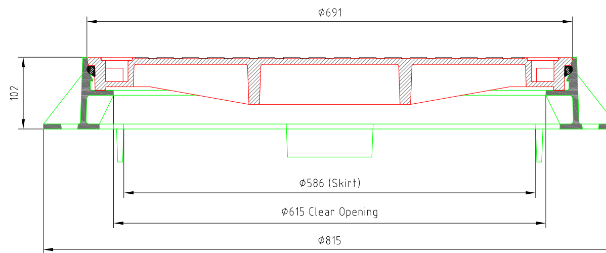
Class 'D' Assembly (73 Kg) With Spigot Frame
