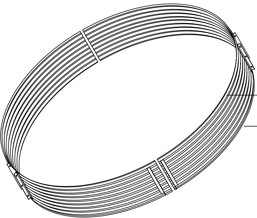
FOUR PIECE COUPLING BAND - MAXI BAND - PIPE φ2850 - φ3600
